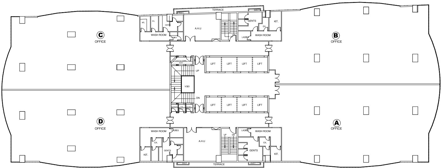
1st TO 14th FLOOR PLAN OFFICES
